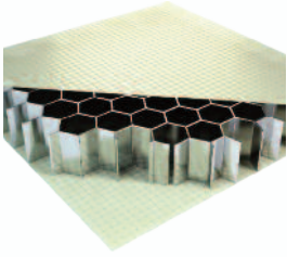
FAH Core made by aluminium honeycomb
